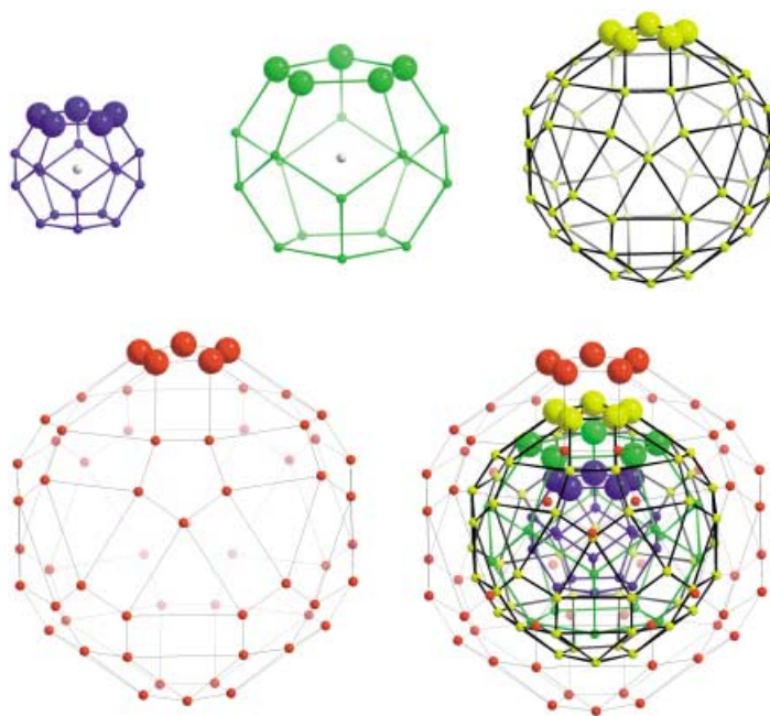
Figure 5. Endohedral hierarchic clusterization of water molecules in the cavity of 2a resulting in \{H_2O\}_{20} dodecahedra (blue and green) and \{H_2O\}_{60} rhombicosidodecahedra (yellow). The second \{H_2O\}_{60} rhombicosidodecahedron (red) is marked out by the 60 H 2 O ligands coordinated to the 12 × 5 Mo atoms of the pentagonal {(Mo)Mo 5 } units. The set of pentagons marked out by the larger spheres highlights that all the pentagons are parallel with the same orientation of the C 5 axes; all the polyhedra have a common center which is indicated by a white sphere, see note added in proof.
